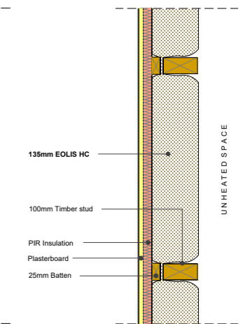
PF376: Ashlar Wall U-value = 0.18 W/m 2 K
