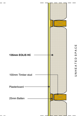
PF375: Ashlar Wall U-value = 0.23 W/m 2 K
