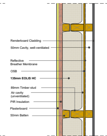
PF350: Timber Frame Wall U-value = 0.18 W/m 2 K
