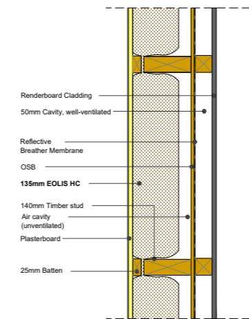
PF347: Timber Frame Wall U-value = 0.22 W/m 2 K
